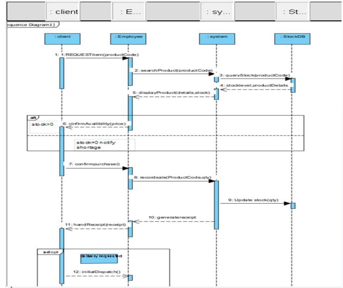
figure 3 SS1 Sequence diagram
