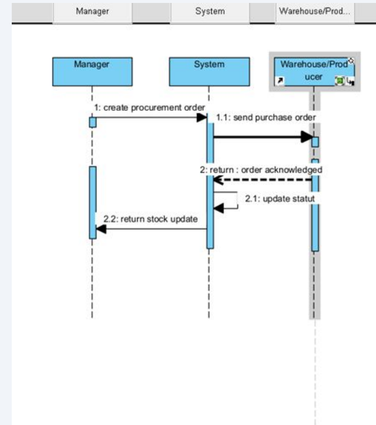
figure 9 SS3 sequence diagram
