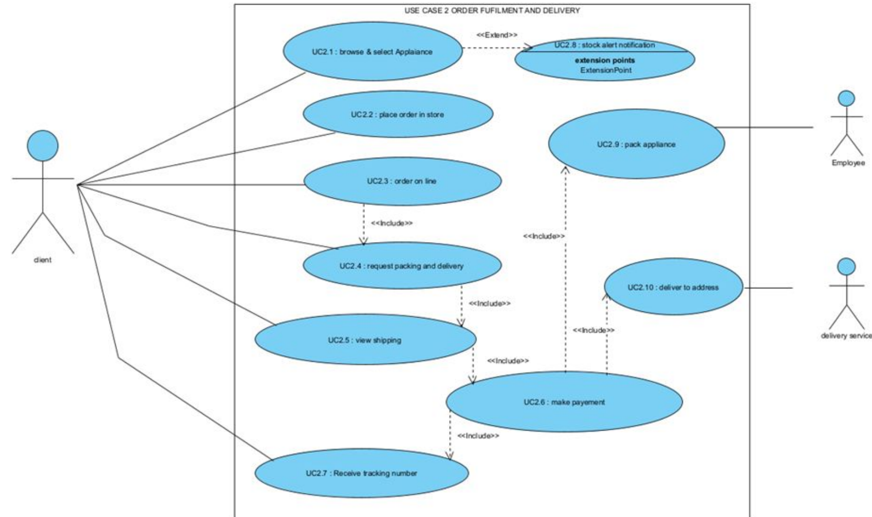
figure 4 SS2 use case diagram
