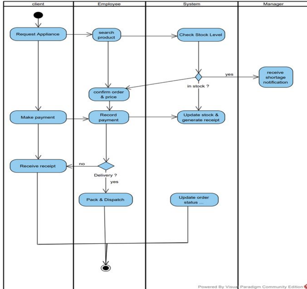
figure 2 SS1 Activity diagram
