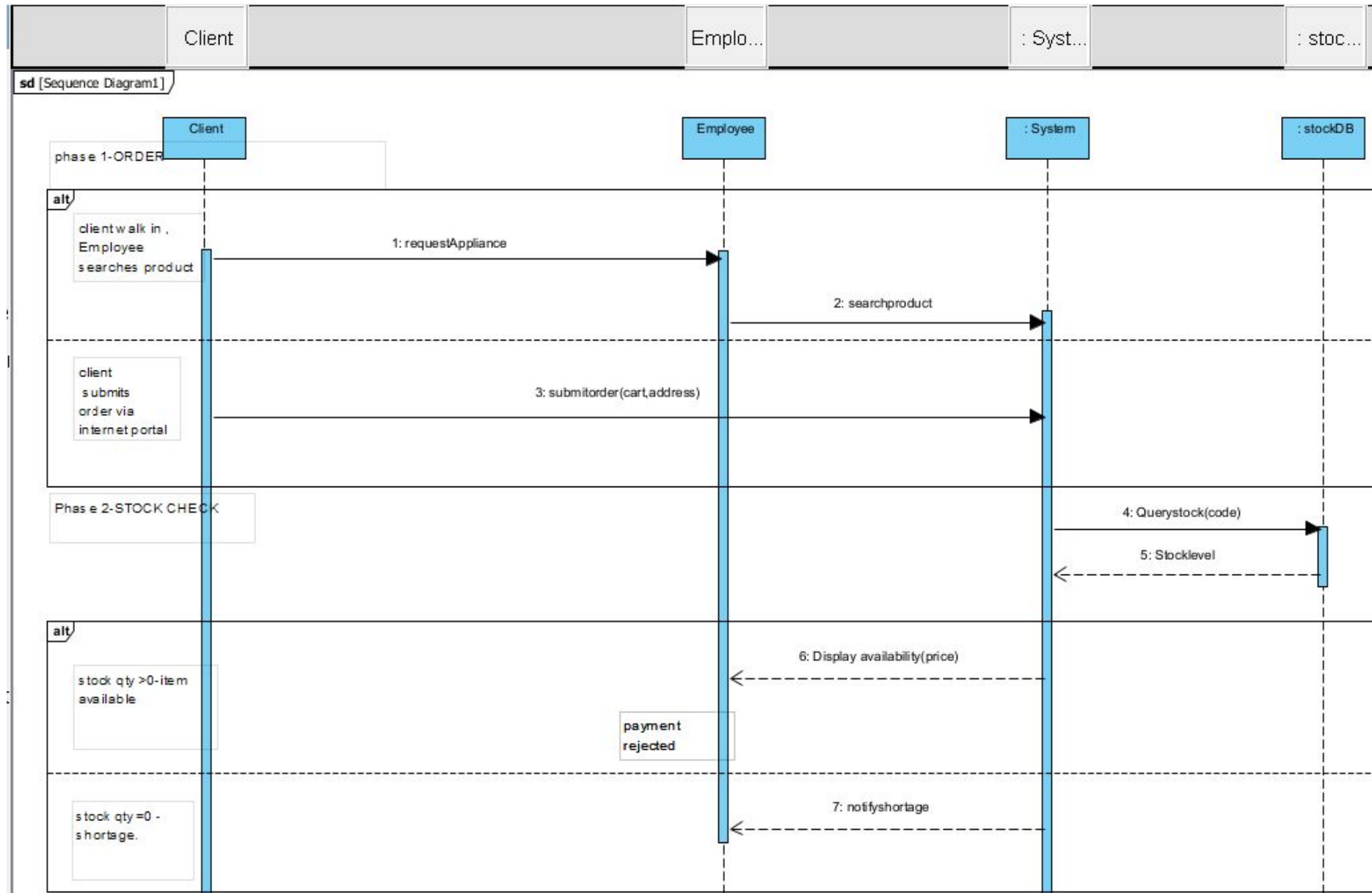
figure 6 SS2 sequence diagram
