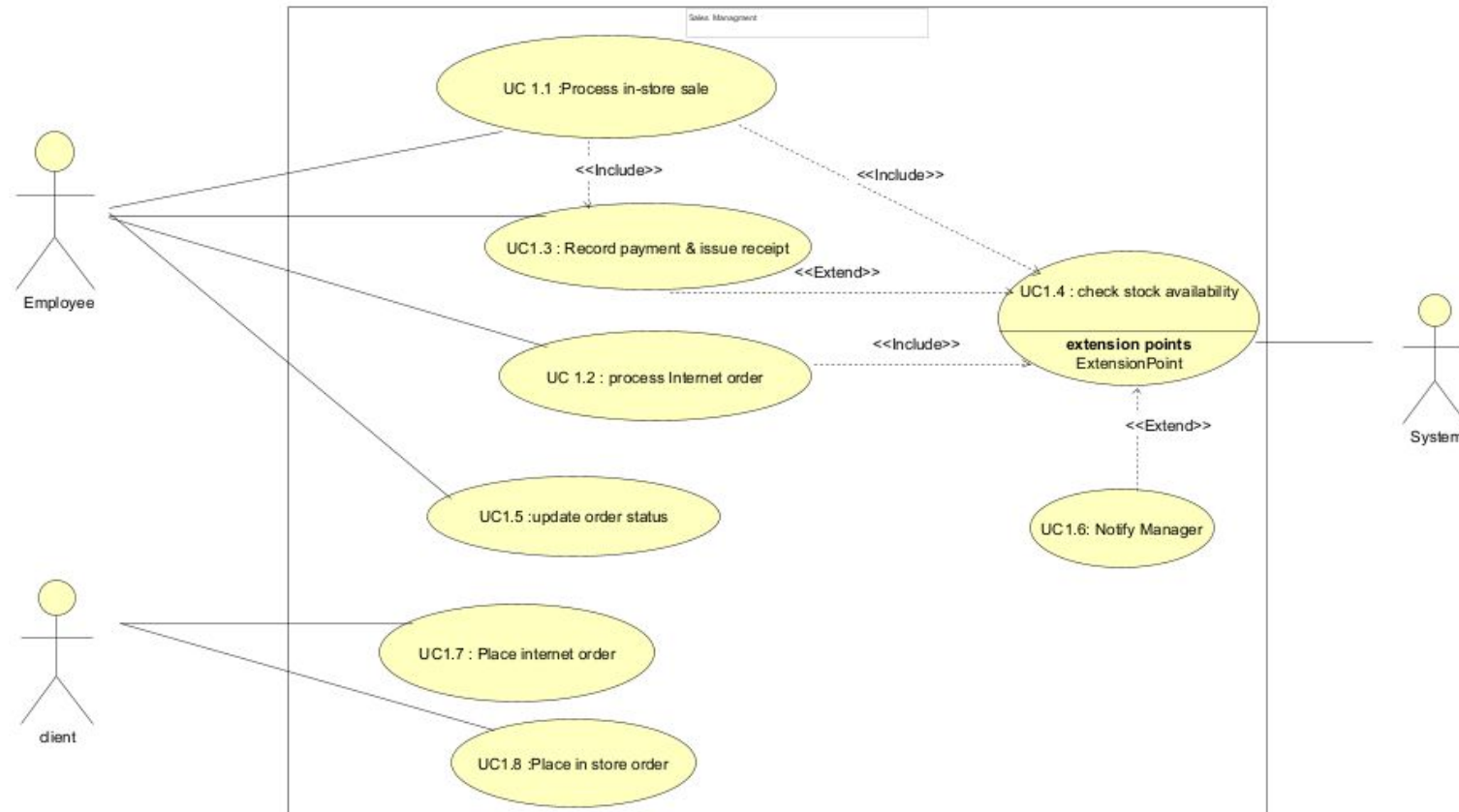
figure 1: ss1 use case diagram
