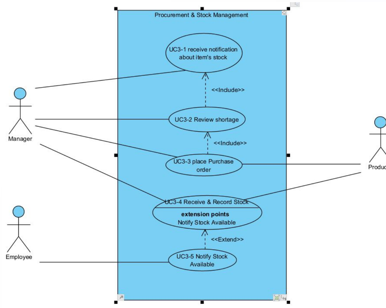
figure 7 SS3 use case diagram
